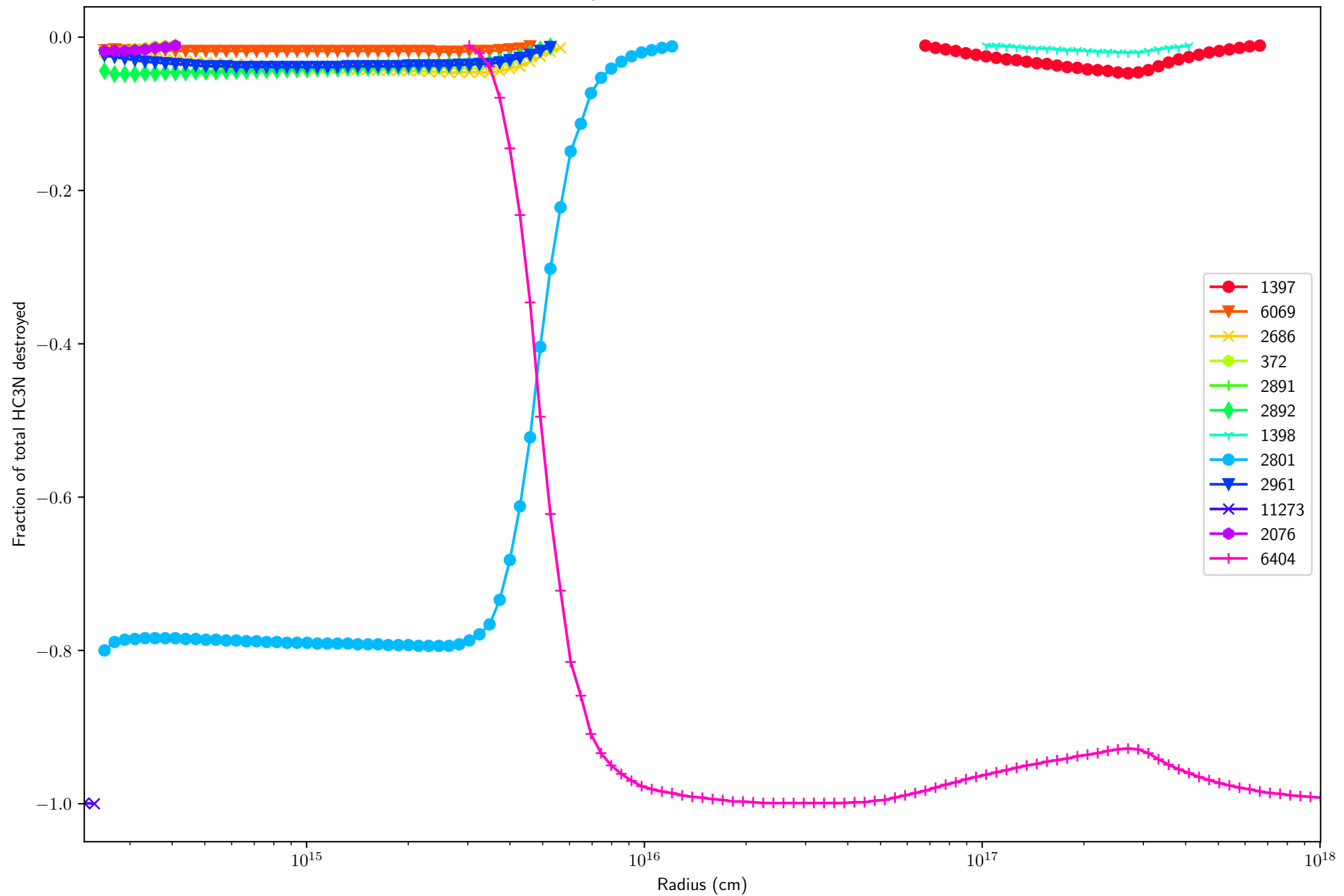
destruction-major-1-HC3N-model-2025-10-15h14-12-29
